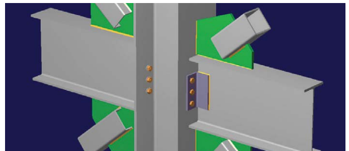
Bracing Connections
