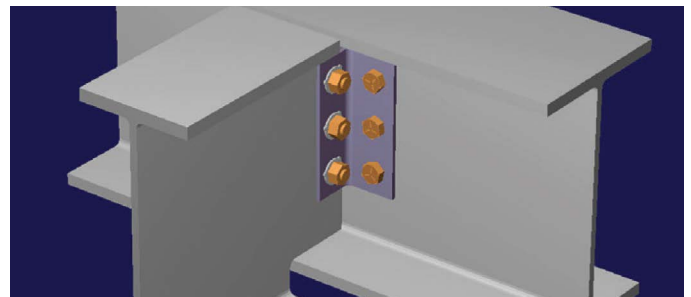
Double-angle Connection
